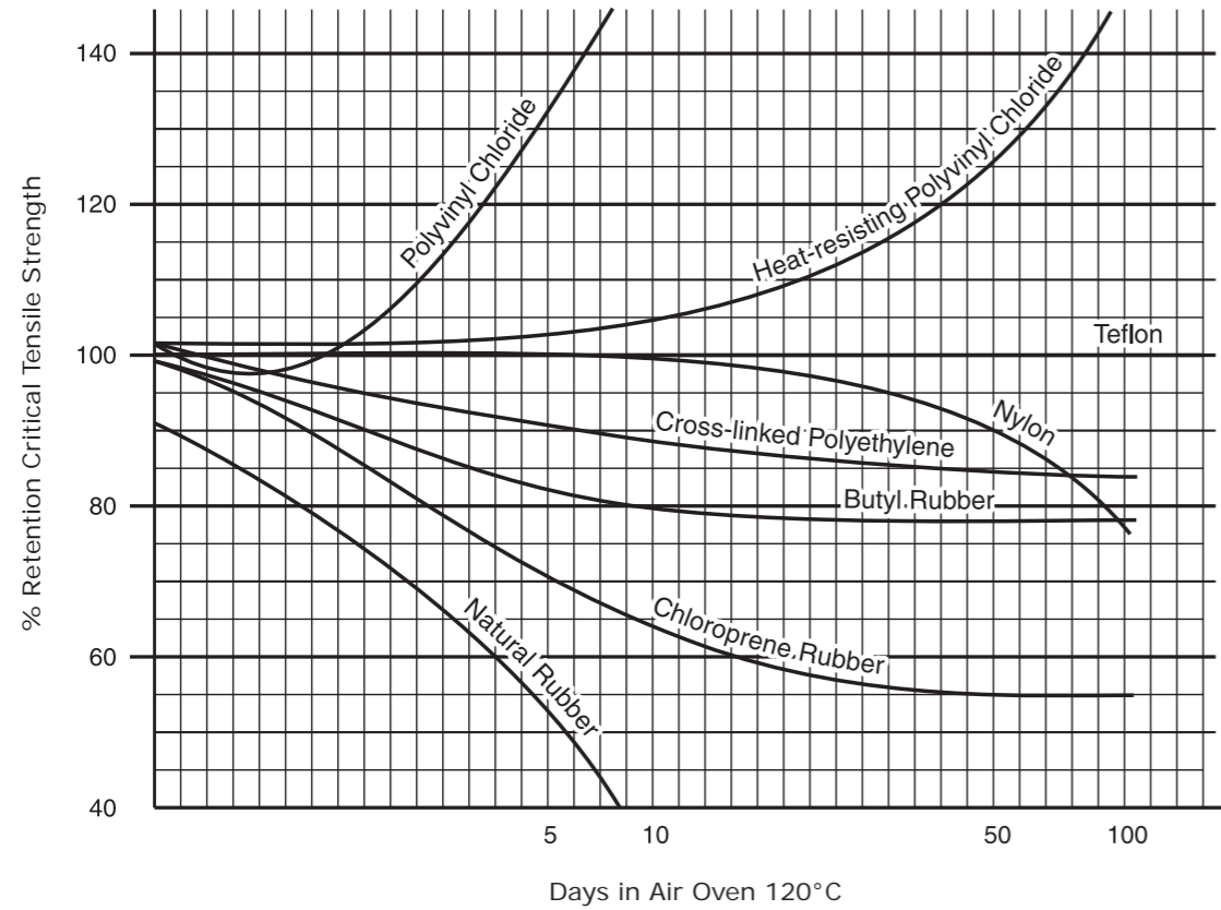
LONG-TIME HEAT AGING CURVES
